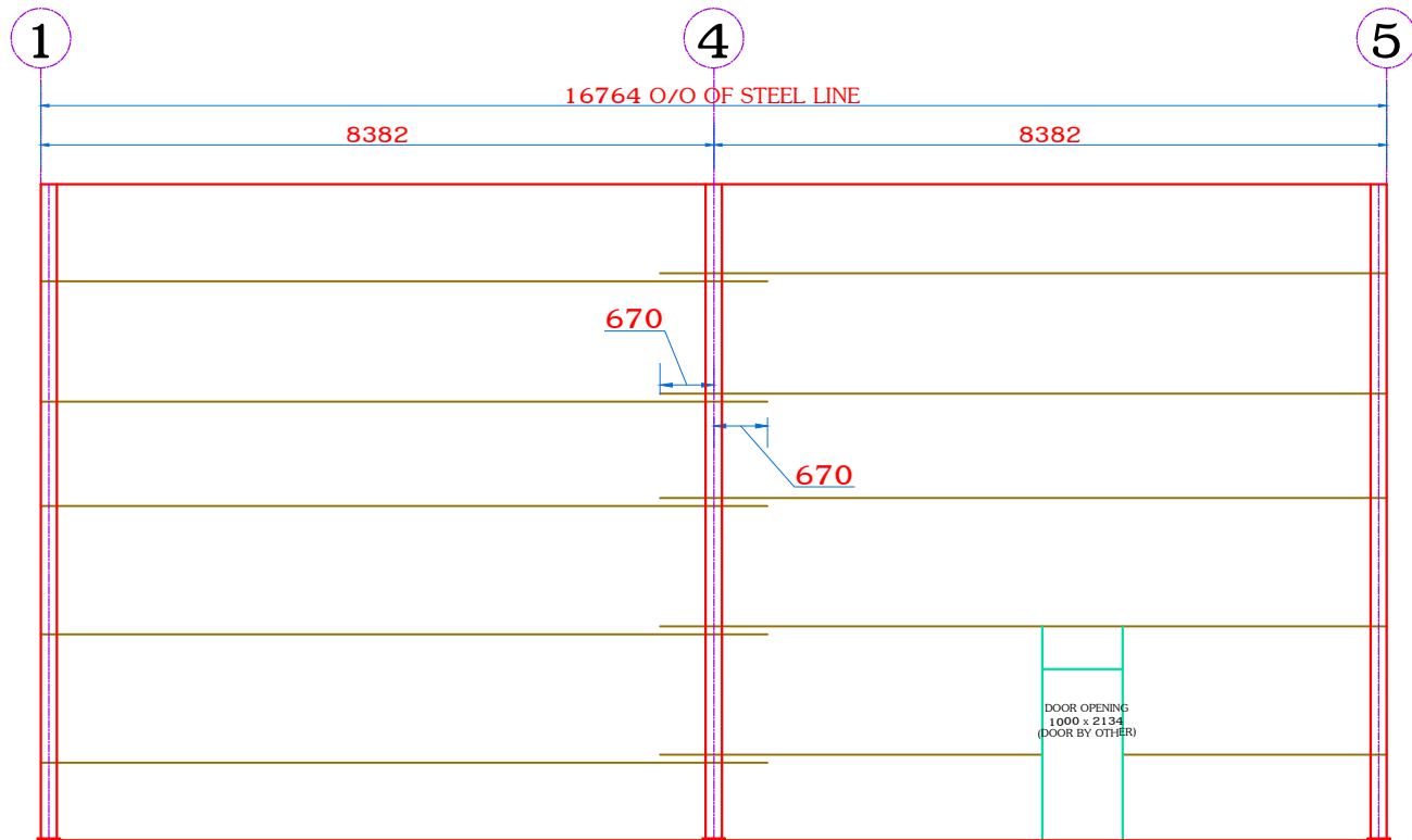
SIDE WALL FRAMING @ GRID-C
