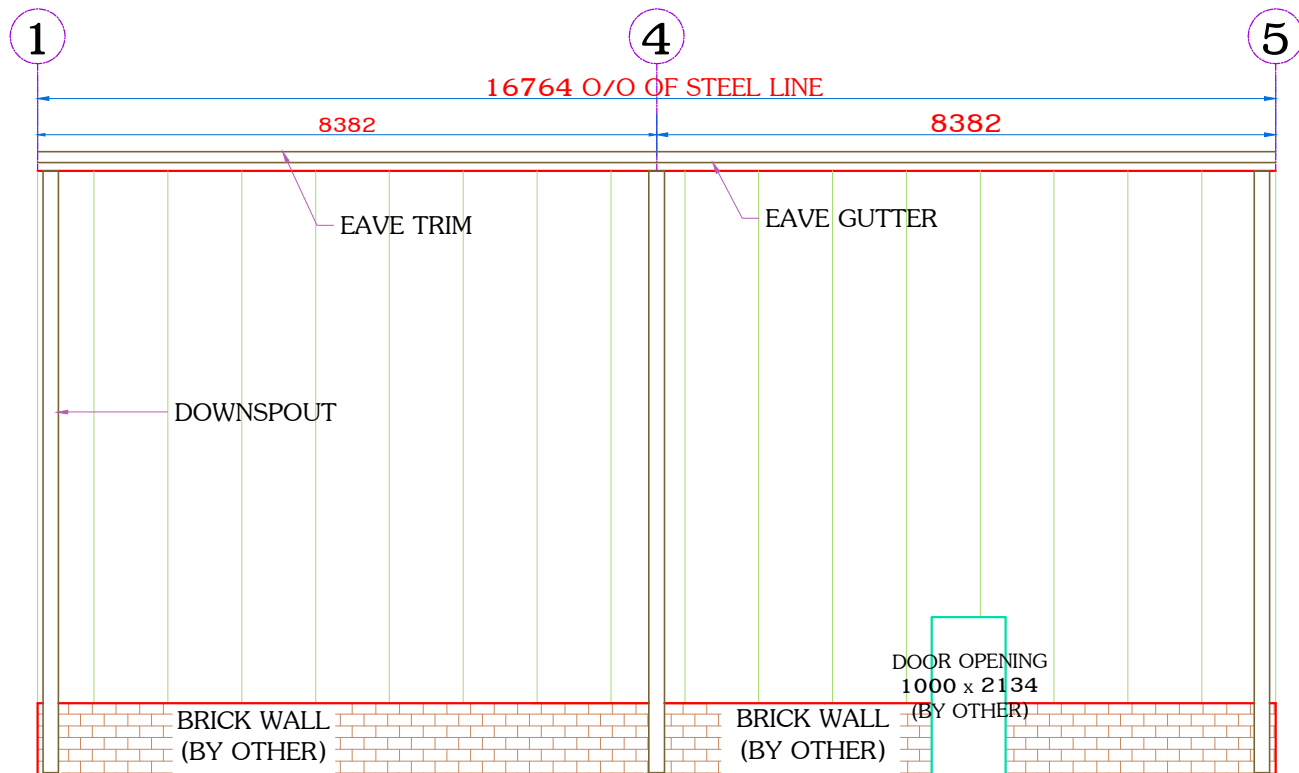
SIDE WALL SHEETING @ GRID-C
